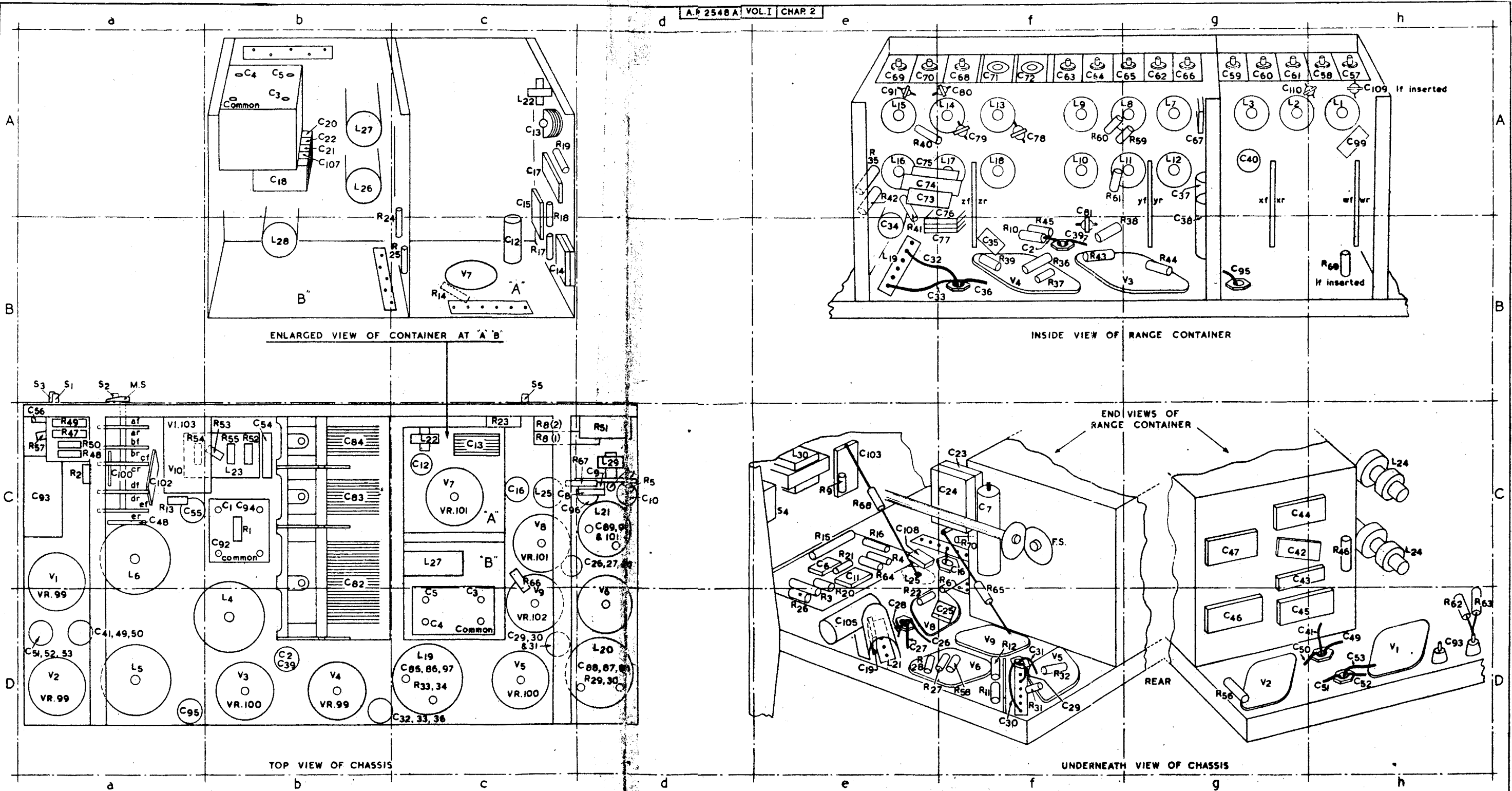
COMPONENTS LOCATION DIAGRAM
