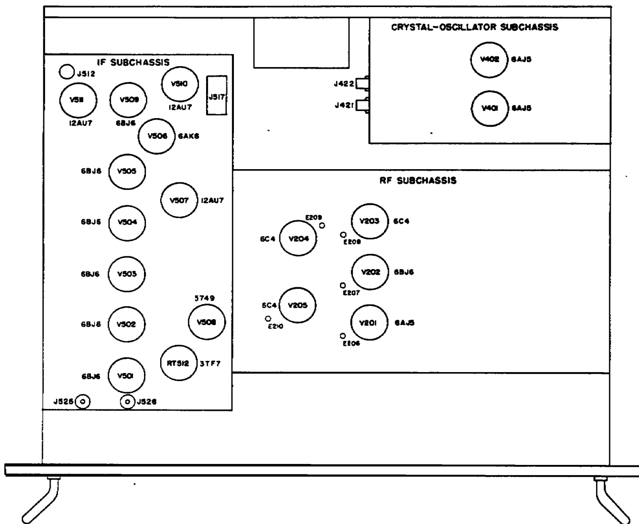
Figure 8. Tube locations, top deck.
