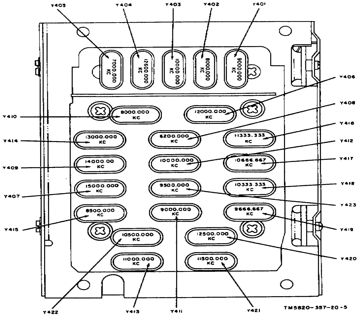
Figure 10. Location of crystals.
