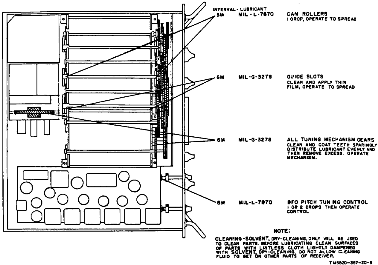
Figure 7. Lubrication.
