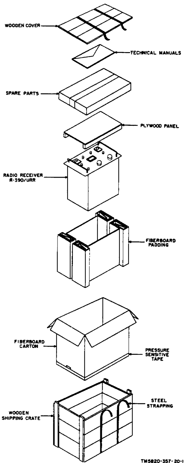
Figure 1. Unpacking
