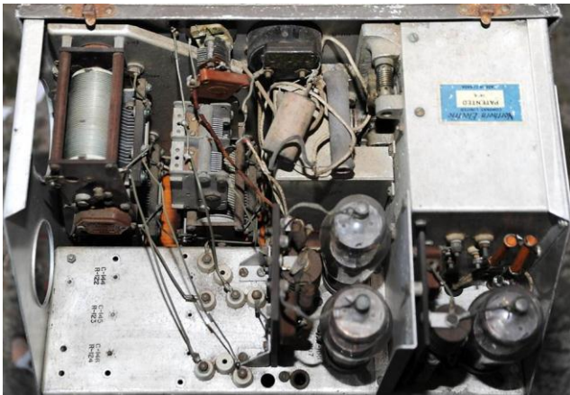
#002 Kachina MP25 HF Packset + Handset
