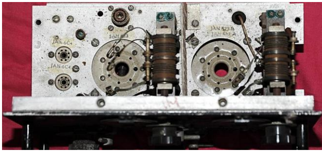
#013 AN/ARC-44 FM TX/RX 24 – 52 MHz with Control Box and Aerial Keyer
