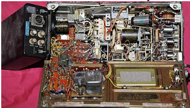
#015 AN/ARC-44 TX/RX unit only
