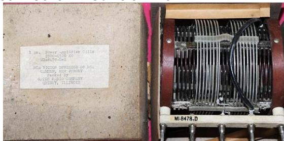
#037 BC610 PA Coil 11 – 15.5 MHz
