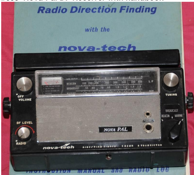
#055 Nova-Pal DF Receiver with handbook
